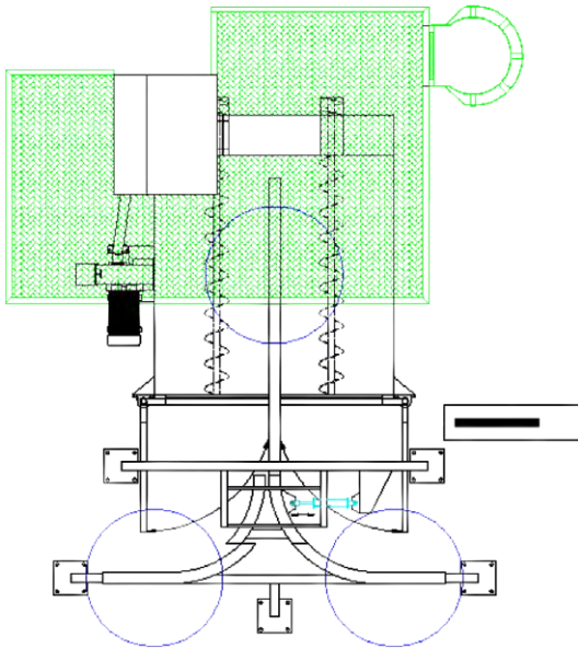
SH 4860Y Top view
