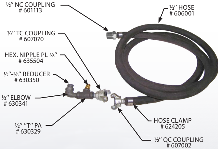
Heavy-Duty hose kit (10' x 1/2") & fittings # 601116
