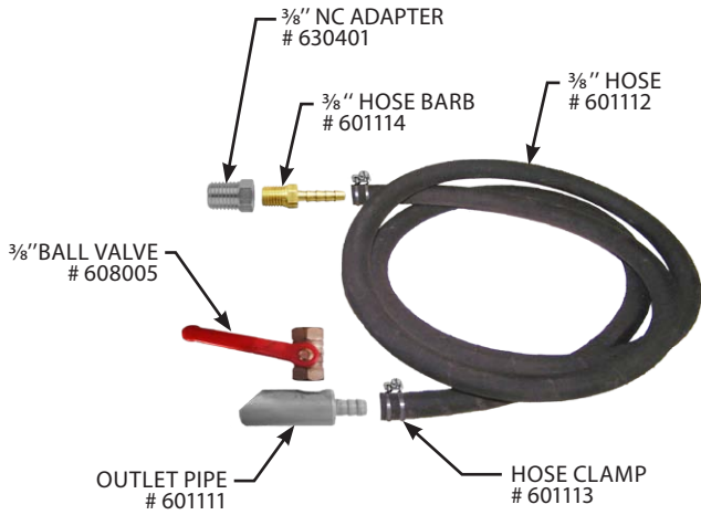
Standard hose kit (8' x 3/8") & fittings
