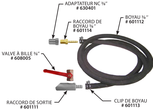
Ensemble de boyau standard (8' x 3/8") & raccords
