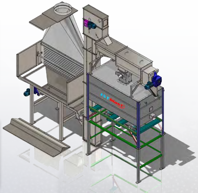
Discharge hopper integrated to the recovery system
